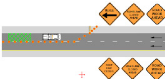
Typical Lane Closure Setup
